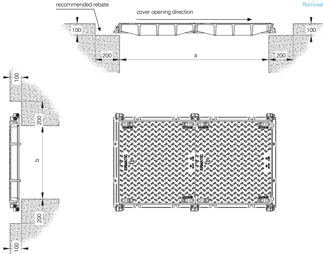
Removable plug cover
